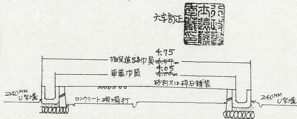
A-A SECTION S=1/50
